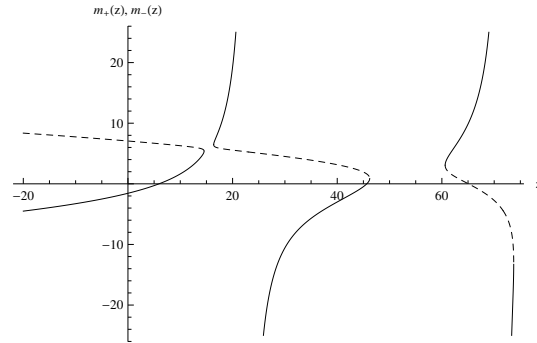
Figure 5.3. The Weyl functions m_+(z) (solid) and m_-(z) (dashed) inside the first three gaps.
